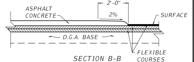
SECTION B-B MOUNTABLE MEDIAN WITH FLEXIBLE PAVEMENT ( TYPE 5 )
