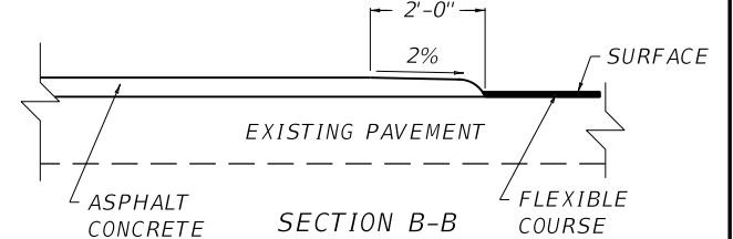
SECTION B-B MOUNTABLE MEDIAN ON EXISTING PAVEMENT ( TYPE 4 )
